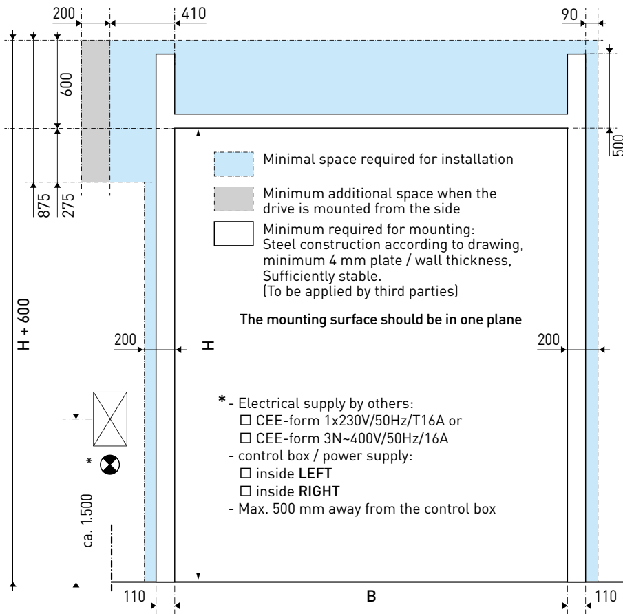
[ Drive side ]
