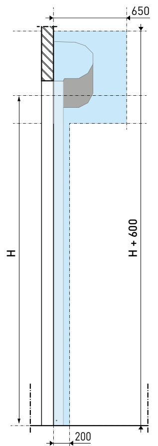
[ Cross section ]
