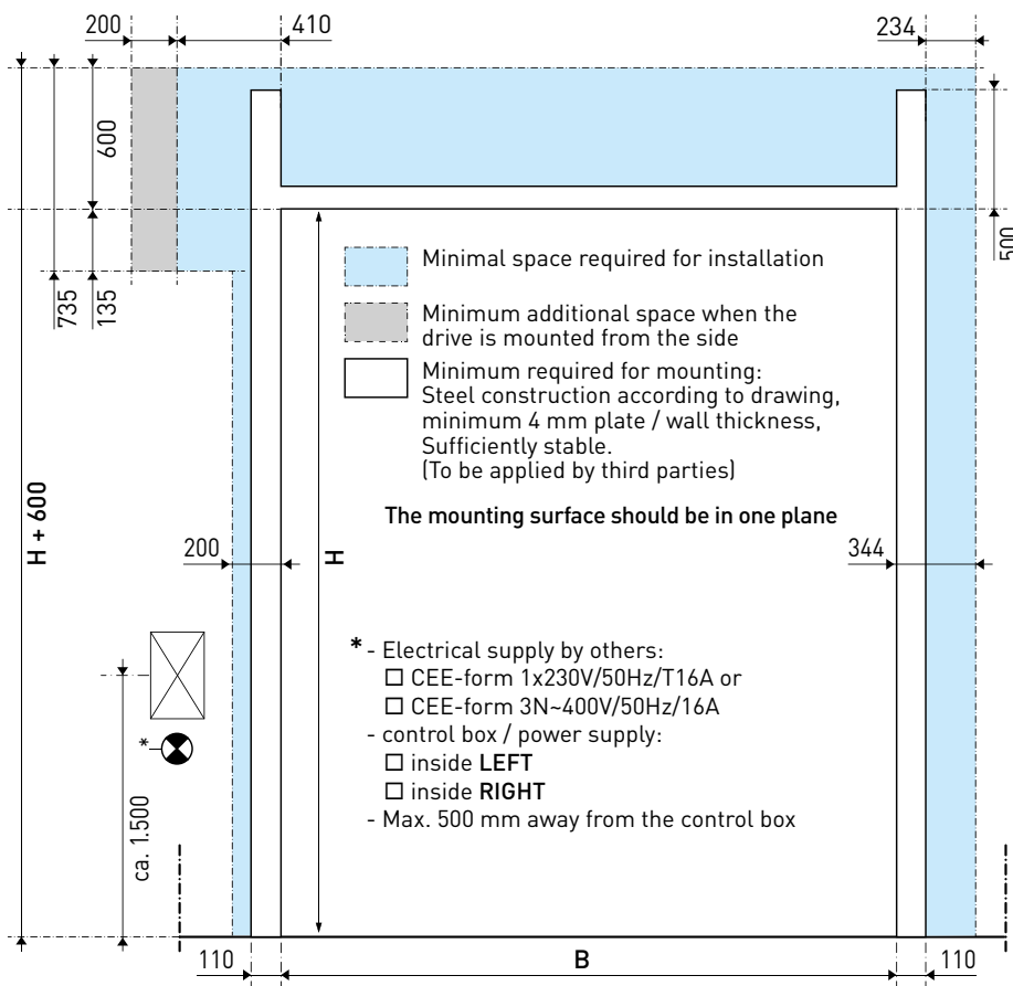
[ Drive side ]
