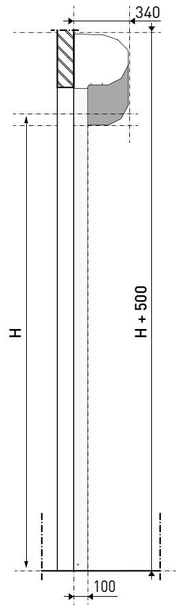
[ Cross section ]
