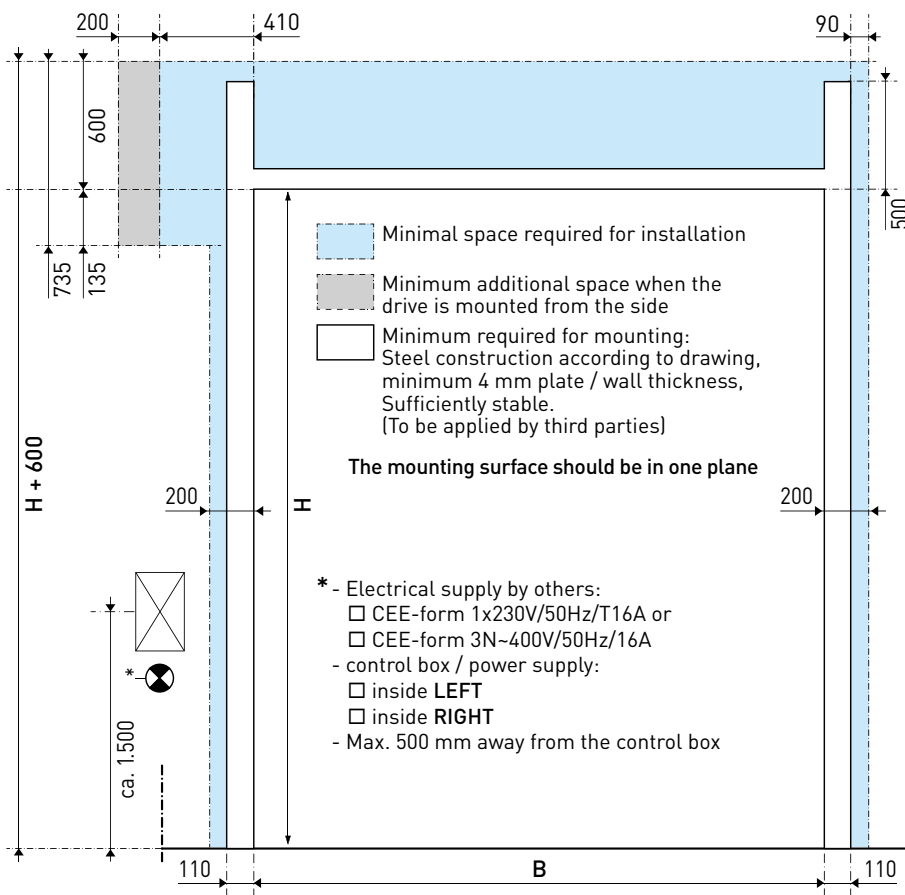
[ Drive side ]
