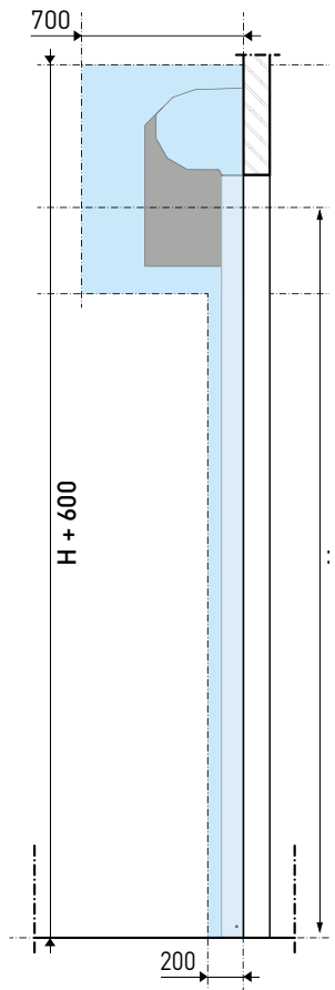
[ Cross section ]
